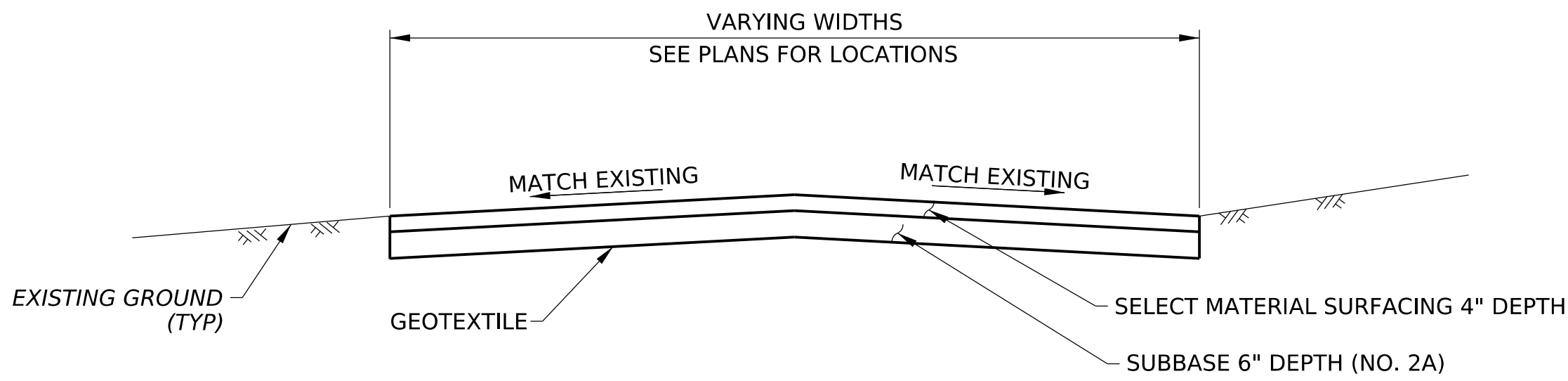
GRAVEL DRIVEWAY SECTION NOT TO SCALE
