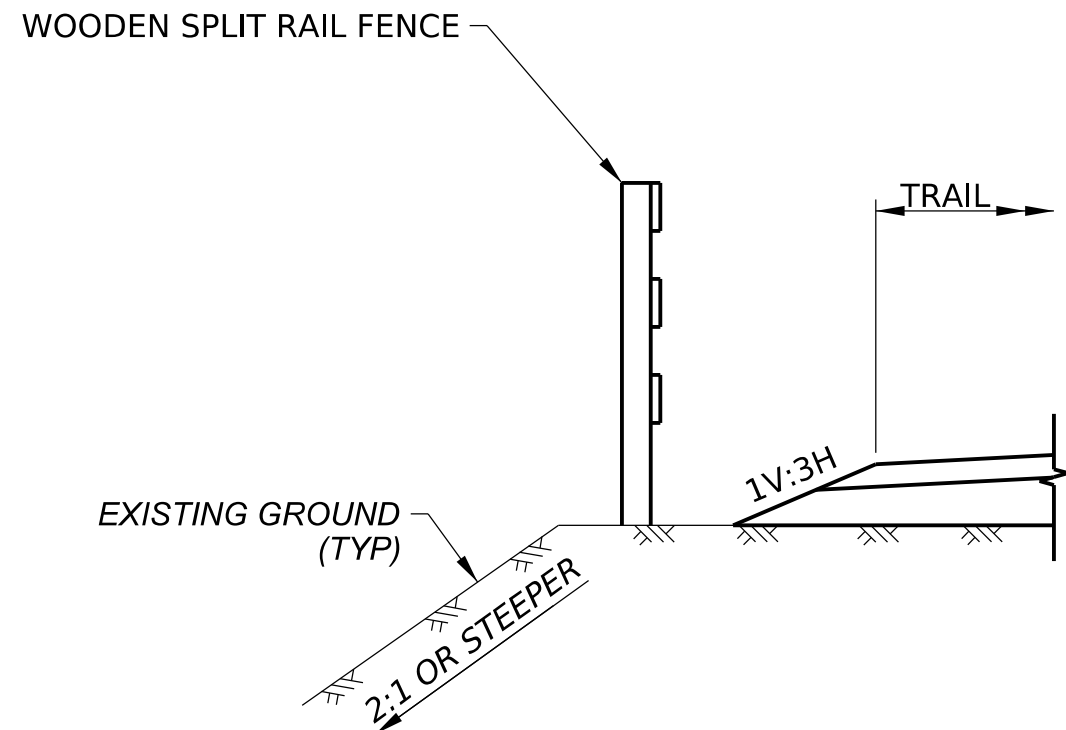
ALTERNATE SECTION NOT TO SCALE STA XXX+XX.XX TO XXX+XX.XX LT
