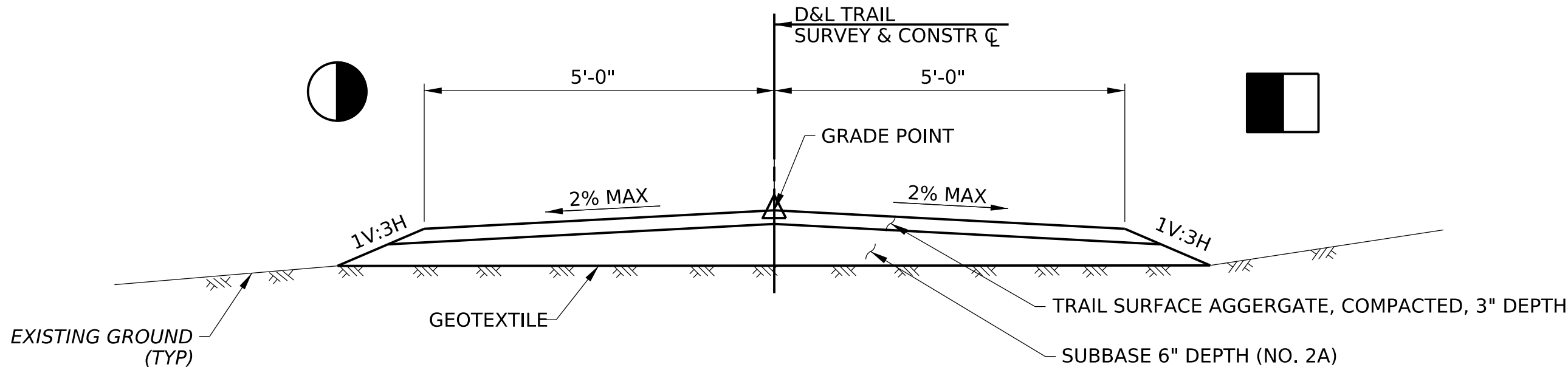
TYPICAL TRAIL SECTION NOT TO SCALE STA 770+35.00 TO STA 792+72.00 STA 799+61.46 TO STA 1016+51.52
