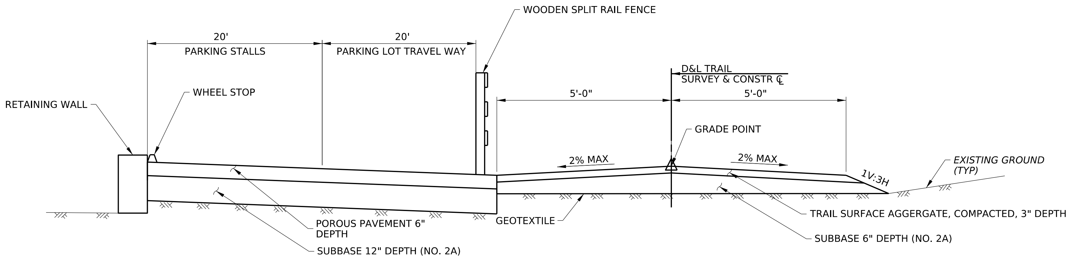
TYPICAL TRAILHEAD PARKING LOT SECTION NOT TO SCALE STA 771+00.00 TO STA 776+25.00
