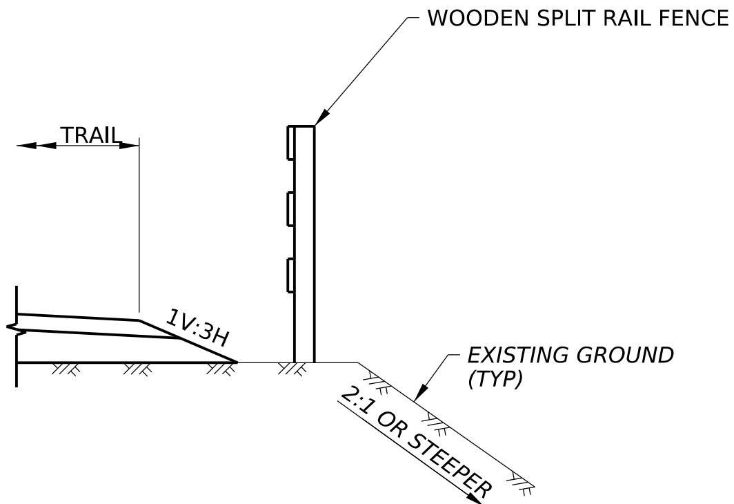
ALTERNATE SECTION NOT TO SCALE STA XXX+XX.XX TO XXX+XX.XX RT
