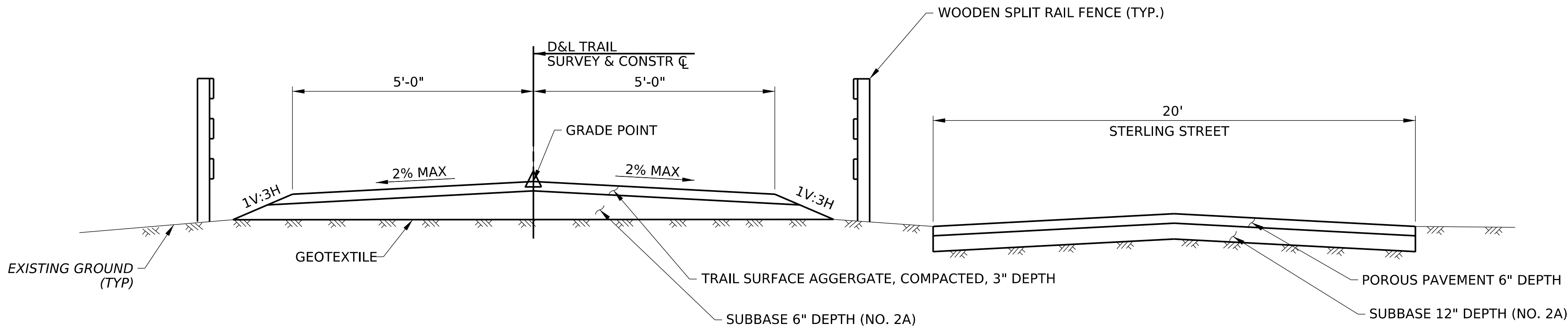
TYPICAL TRAIL SECTION AT STERLING STREET NOT TO SCALE STA 793+50.00 TO STA 794+75.00
